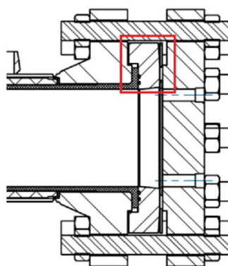
High Performance Compression Ring
